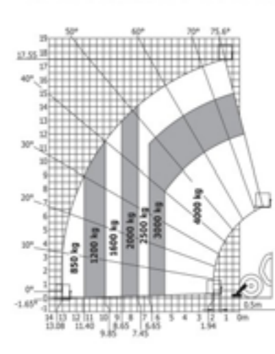
Machine on lowered stabilisers with forks Metric
