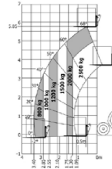
Machine on tires with forks - with levelling device Metric
