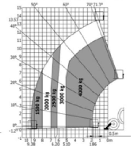
Machine on lowered stabilisers with forks Metric
